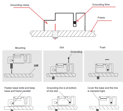
Figure 14 Clamp Grounding Method
